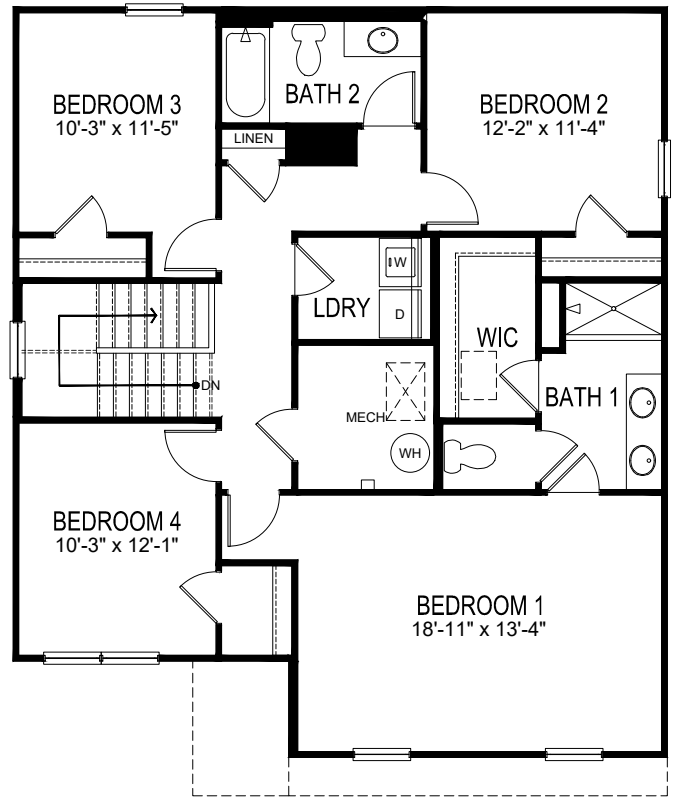
SECOND FLOOR
