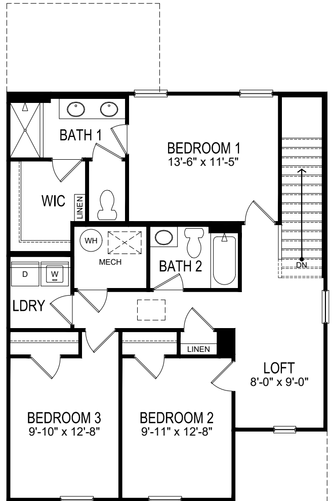
SECOND FLOOR
