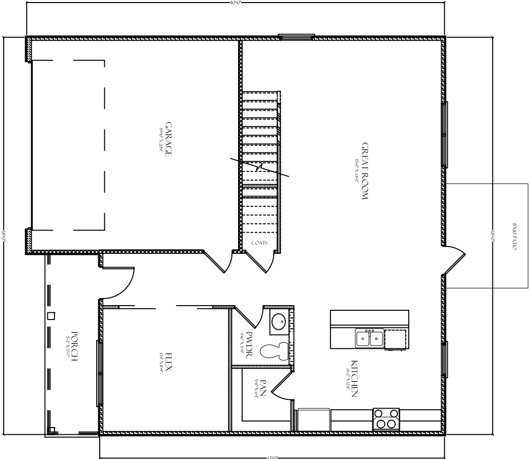
1 | FIRST FLOOR PLAN SCALE: 1/4" = 1'-0"
