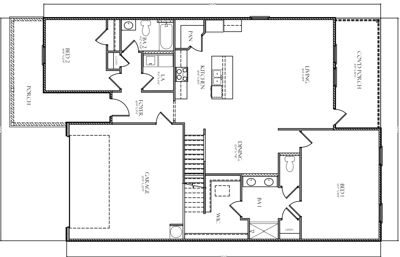
1 FIRST FLOOR PLAN - OZARK C SCALE: 1/8" = 1'-0"
