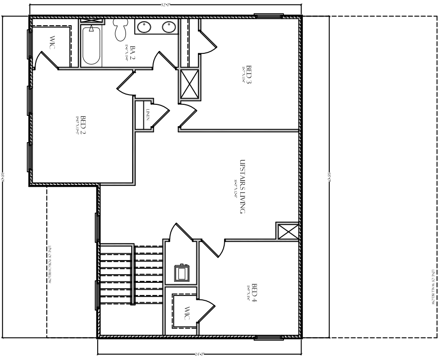
2 SECOND FLOOR PLAN SCALE: 1/4" = 1'-0"
