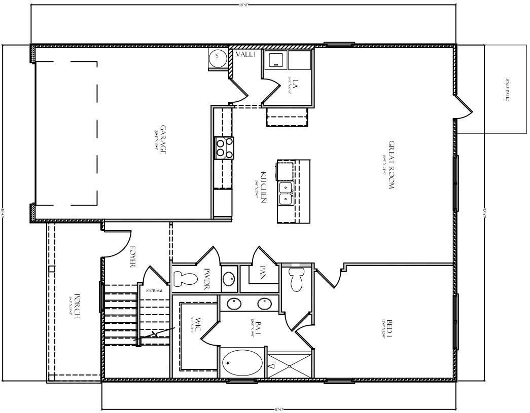
1 FIRST FLOOR PLAN SCALE: 1/4" = 1'-0"
