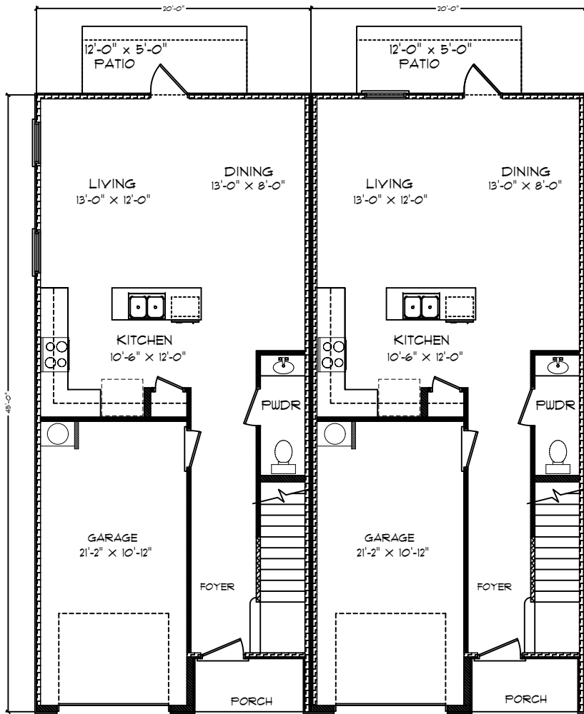
1ST FLOOR PLAN - EXTERIOR PALM TOWNHOME - PC 4 TALLY
