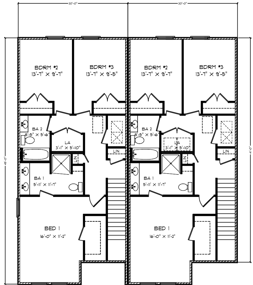
2ND FLOOR PLAN - EXTERIOR PALM TOWNHOME - PC 4 TALLY
