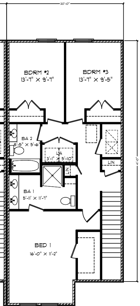
2ND FLOOR PLAN - INTERIOR PALM TOWNHOME - PC 4 TALLY
